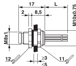
Dimensional drawing
